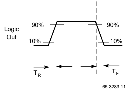
Figure 8. Rise/Fall Times
